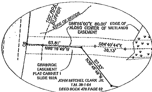
DETAIL 1"=30'
